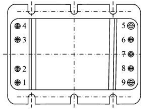
Fig 5 Upward view
