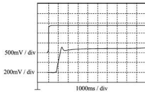
Figure 5 Start-up overshoot/ delay
