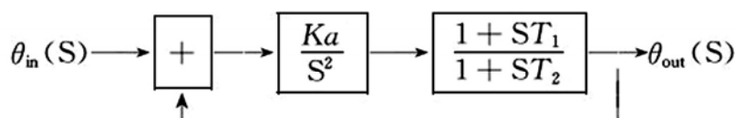
Fig.2 Block diagram of operating principle
