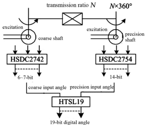
Fig. 9 Application of SDC Two-Speed System
