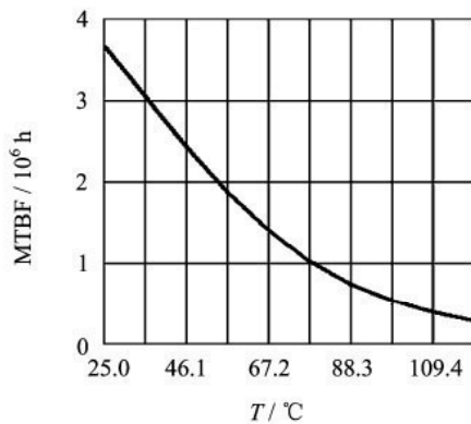
Fig.7 MTBF-Temperature Curve
