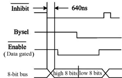
Fig. 4 Time sequence chart for 8-bit bus transfer
