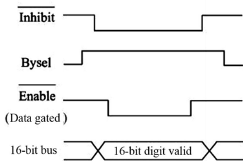
Fig. 3 Time sequence chart for 16-bit bus transfer
