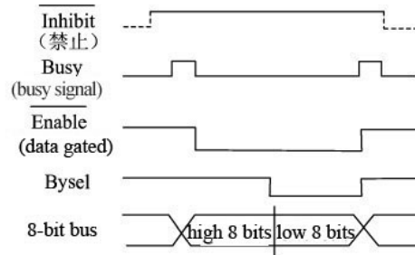
Fig. 6 Time sequence of 8-bit bus transfer
