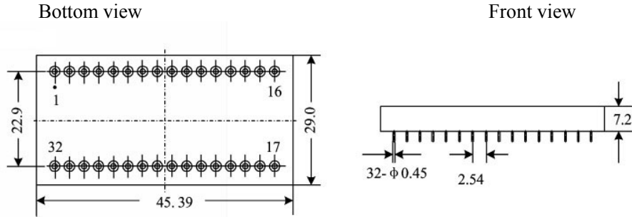
Fig.10 Outside view of package
