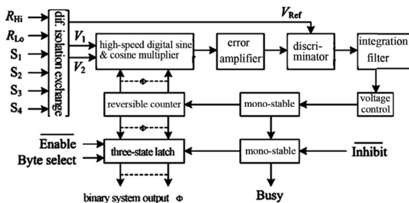
Fig.2 Block diagram of operating principle
