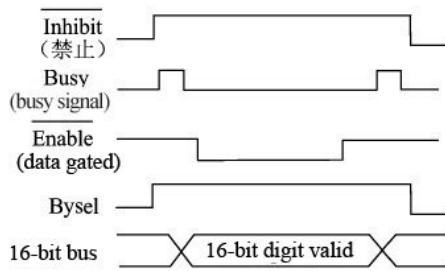
Fig. 5 Time sequence of 16-bit bus transfer
