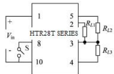
Figure 19 Application Connection Diagram for Triple output models
