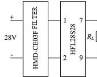
Figure 19 Connection Diagram for Model HFL28S28 Converter with EMI Filter
