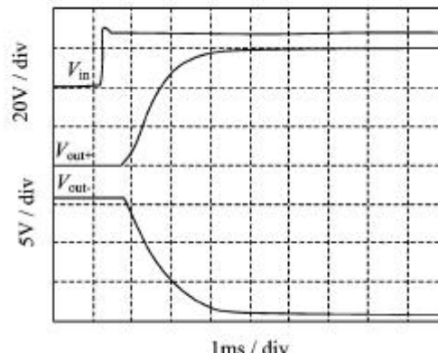
Figure 9 START-UP OVERSHOOT/DELAY
